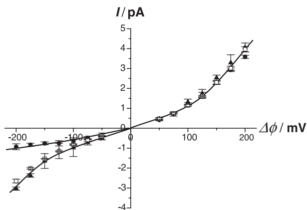
Fig. 5. Current–voltage curves of single SRE channels in DPhPC membranes in the absence of PG (□) and in the presence of PG (10 μM) on the cis -side (●) and on the trans -side (▲). Membranes were bathed by 0.1 M NaCl (pH 6) solution.
