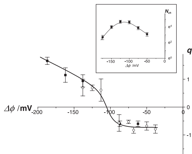
Fig. 4. Potential dependence of the q values of SRE channels in membranes formed from DOPS (■) and from equimolar mixtures of DOPS and DOPE (○). The membrane-bathing solution was 1 M NaCl (pH 6). Insert: Dependence of the number of open SRE channels on the transmembrane potential. Membranes were prepared from DOPS and bathed in 1 M NaCl (pH 6).
